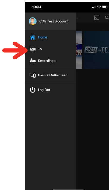
Navigation Bar
