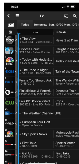
Channel Lineup
